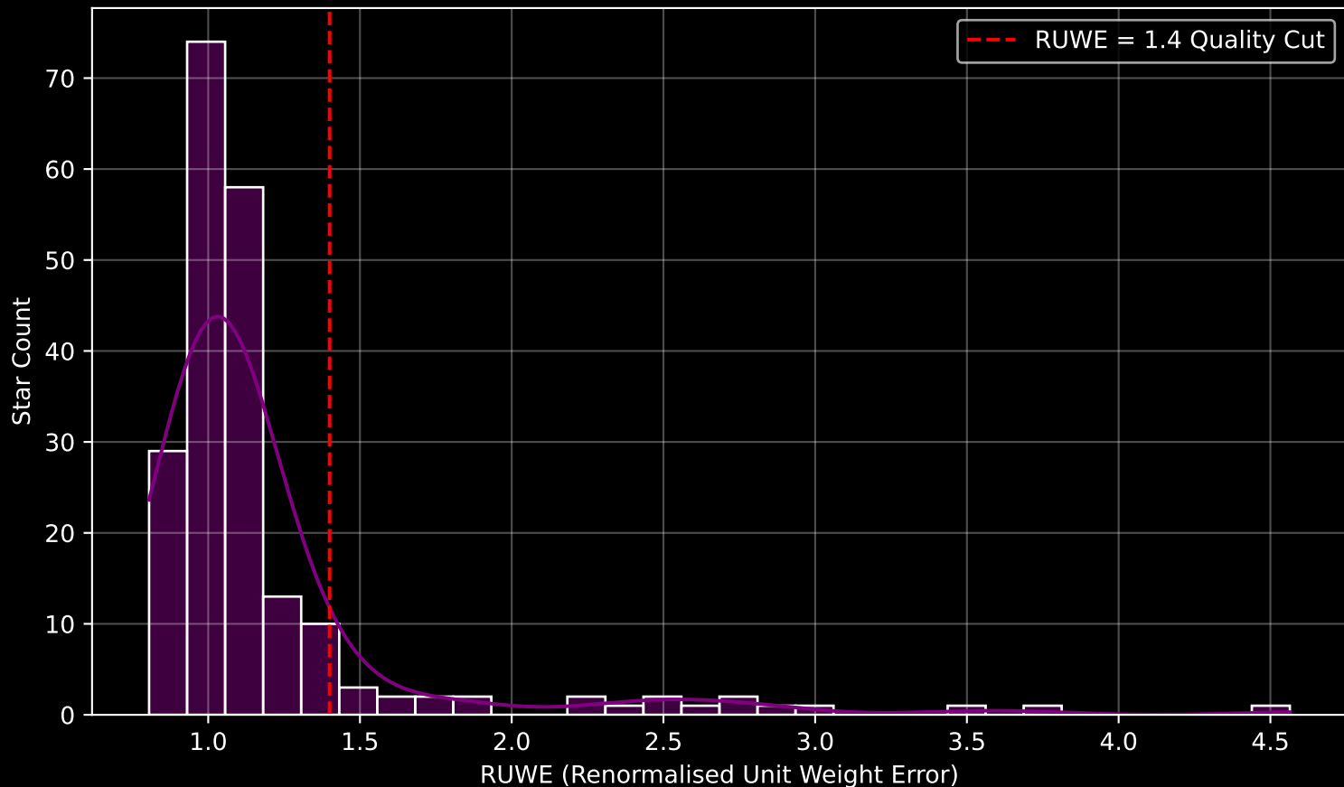
GAPOGEE DR17 Field [170-60] RUWE Distribution (n= 206)
