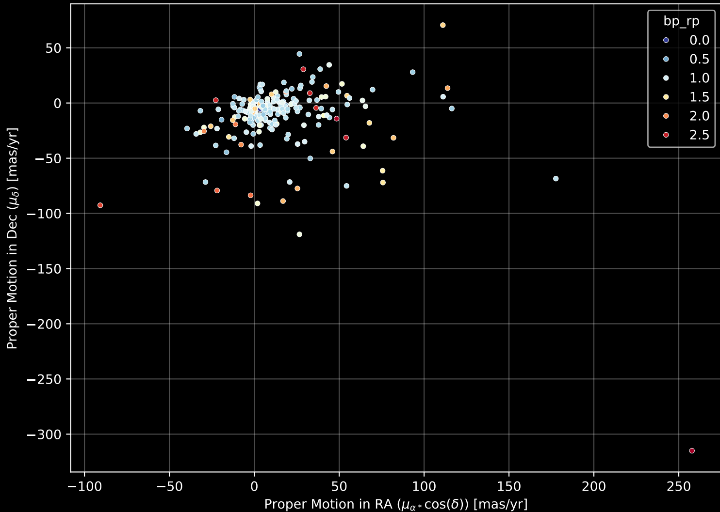
APOGEE DR17 Field: [170-60] Proper Motion Diagram (n= 219)
