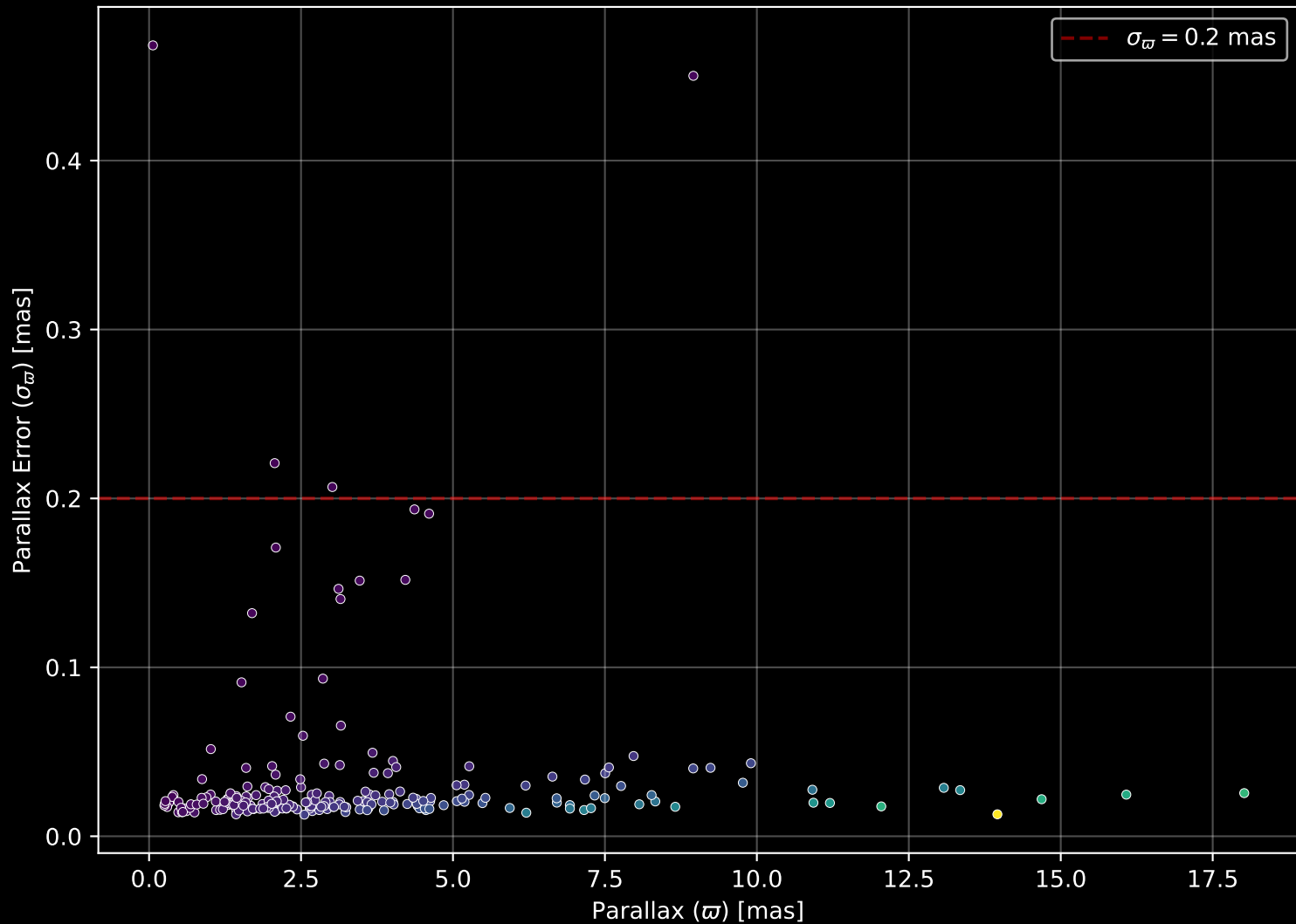
APOGEE DR17 Field: [170-60] Parallax Quality (n= 219)
