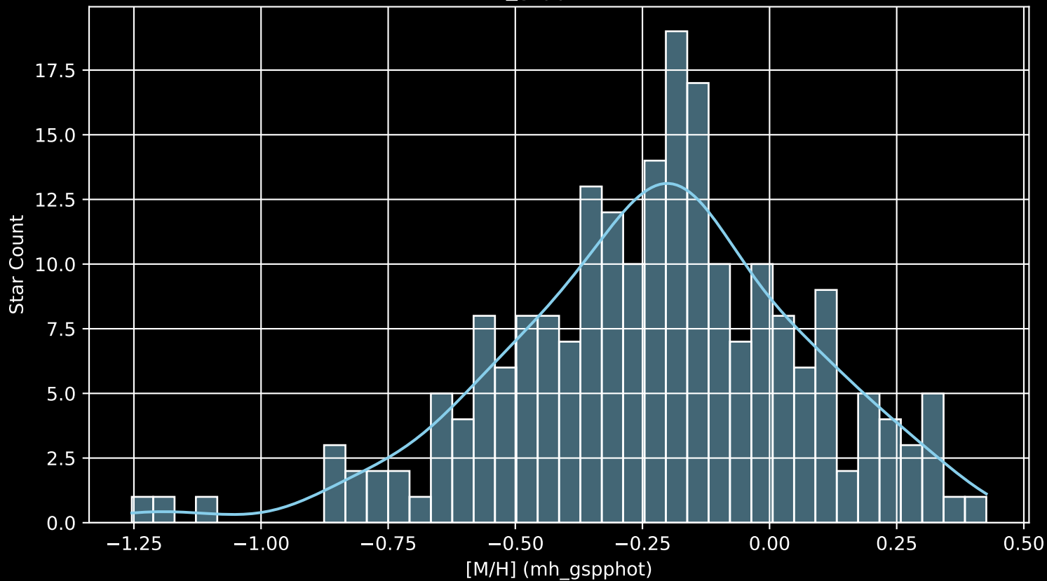
APOGEE DR17 Field: [170-60 [M/H] (mh_gspphot) (n= 215)
